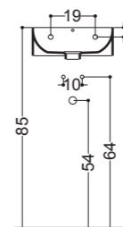
Lavabo 02C 02C Basin 35x35 cm
