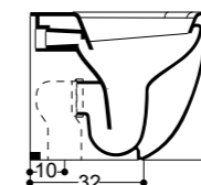
Vaso Terra BTW Wc 34x52 cm
