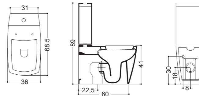
Vaso Monoblocco Longer BTW Monobloc Wc Longer 36x68,5 cm
