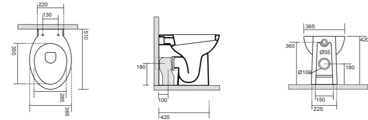
Vaso Terra BTW Wc 36,5x51 cm
