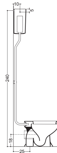
Art 06050 Cassetta Alta High level cistern 38x45,5 cm
