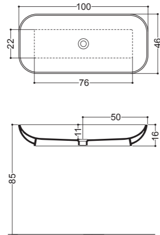
Lavabo Appoggio Overtop Basin 100x46 cm
