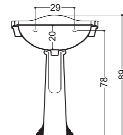
Lavabo Basin 64x48 cm
