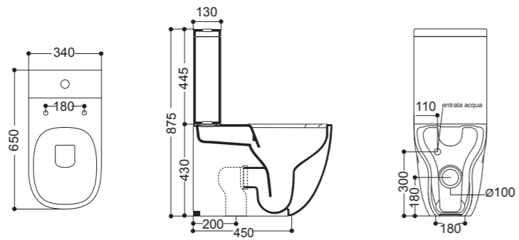
Vaso Monoblocco NoRim BTW Monobloc Wc NoRim 34x65 cm
