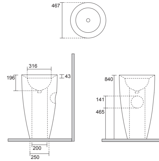
Lavabo Freestanding Parete Freestanding Washbasin Wall Ø 46 cm
