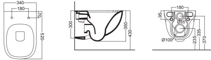
Vaso Sospeso NoRim Wall-hung Wc NoRim 34x52 cm
