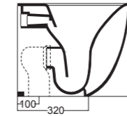
Vaso Terra NoRim BTW Wc NoRim 34x52 cm
