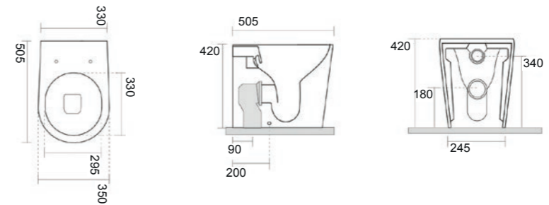
Vaso Terra BTW Wc 33x50 cm
