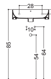
NET Lavabo NET Basin 45x35 cm
