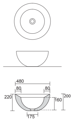
Lavabo Appoggio 200 Counter Top Washbasin 200 \varnothing 48 cm
