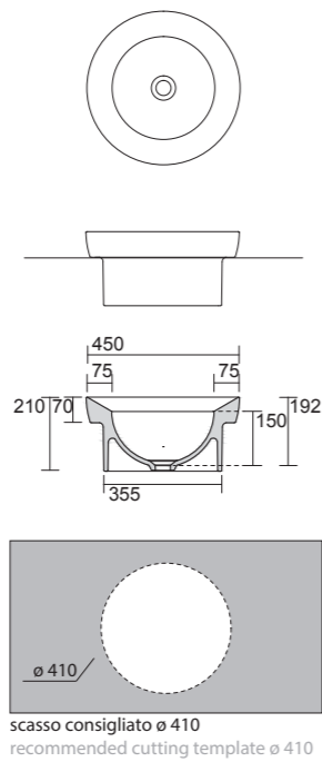
Lavabo Incasso 70 Inset Washbasin 70 \varnothing 45 cm
