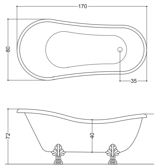
Vasca Bathtub 170x80 cm
