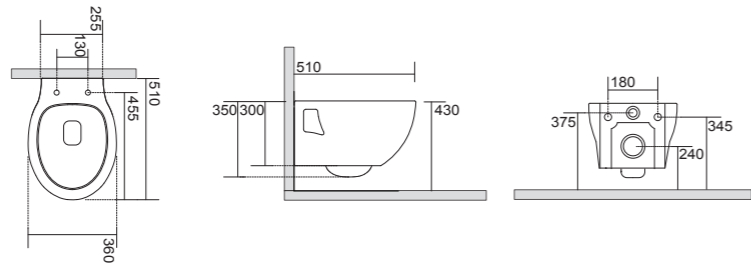
Vaso Sospeso Wall-hung Wc 37,5x51 cm
