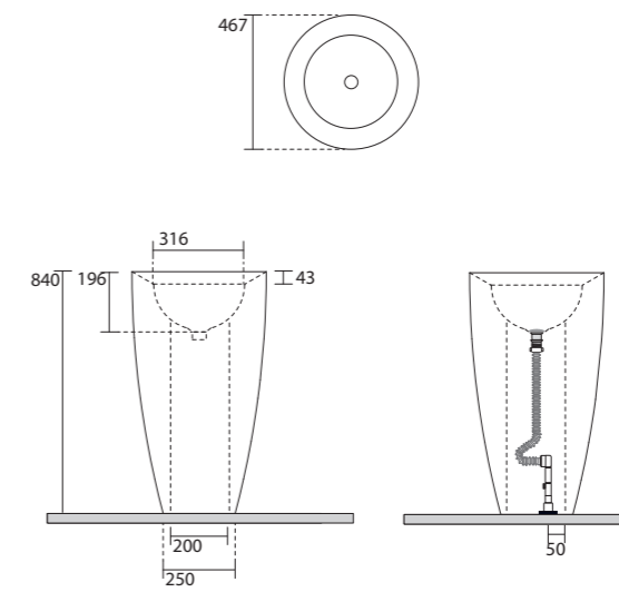
Lavabo Freestanding Terra Freestanding Washbasin Floor Ø 46 cm
