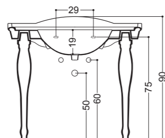
Consolle Console 100x45 cm
