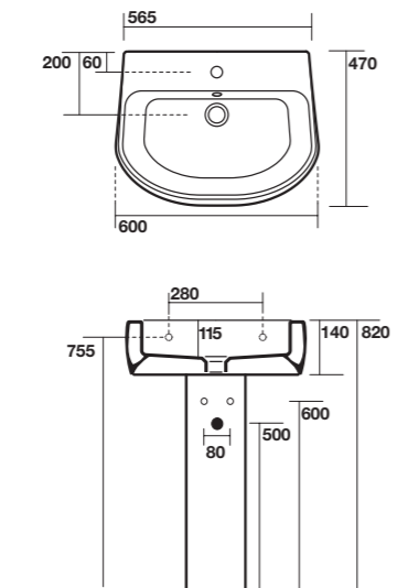
Lavabo Sospeso o Colonna Wall-hung or on Pedestal Basin 60x47 cm
